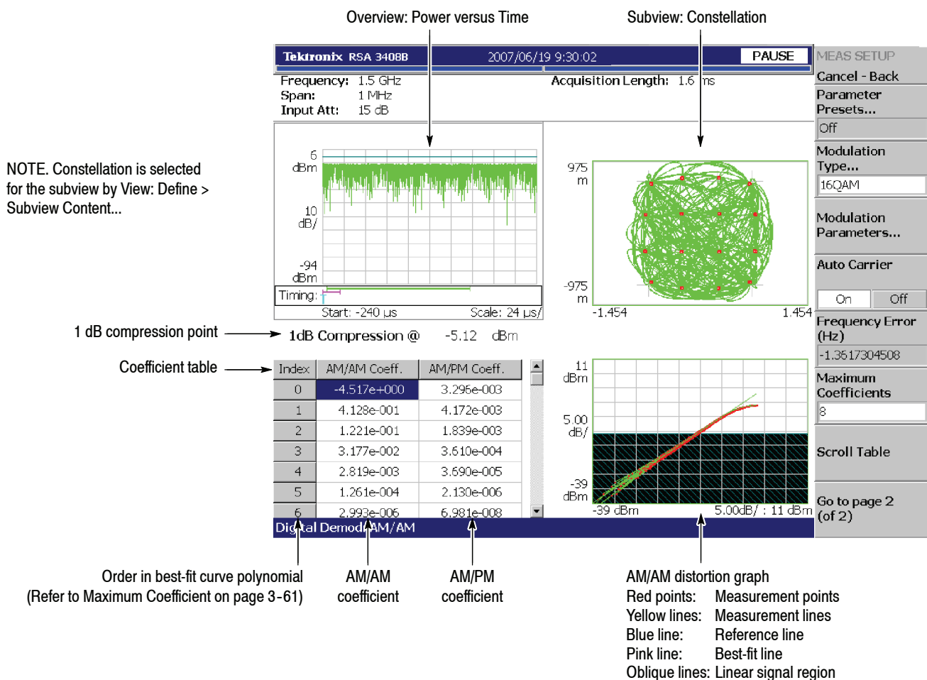
Figure 3-52: AM/AM measurement
