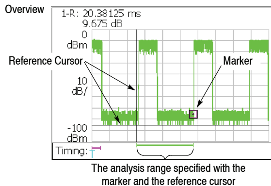
Figure 3-34: Specifying the range with the marker and the reference cursor
