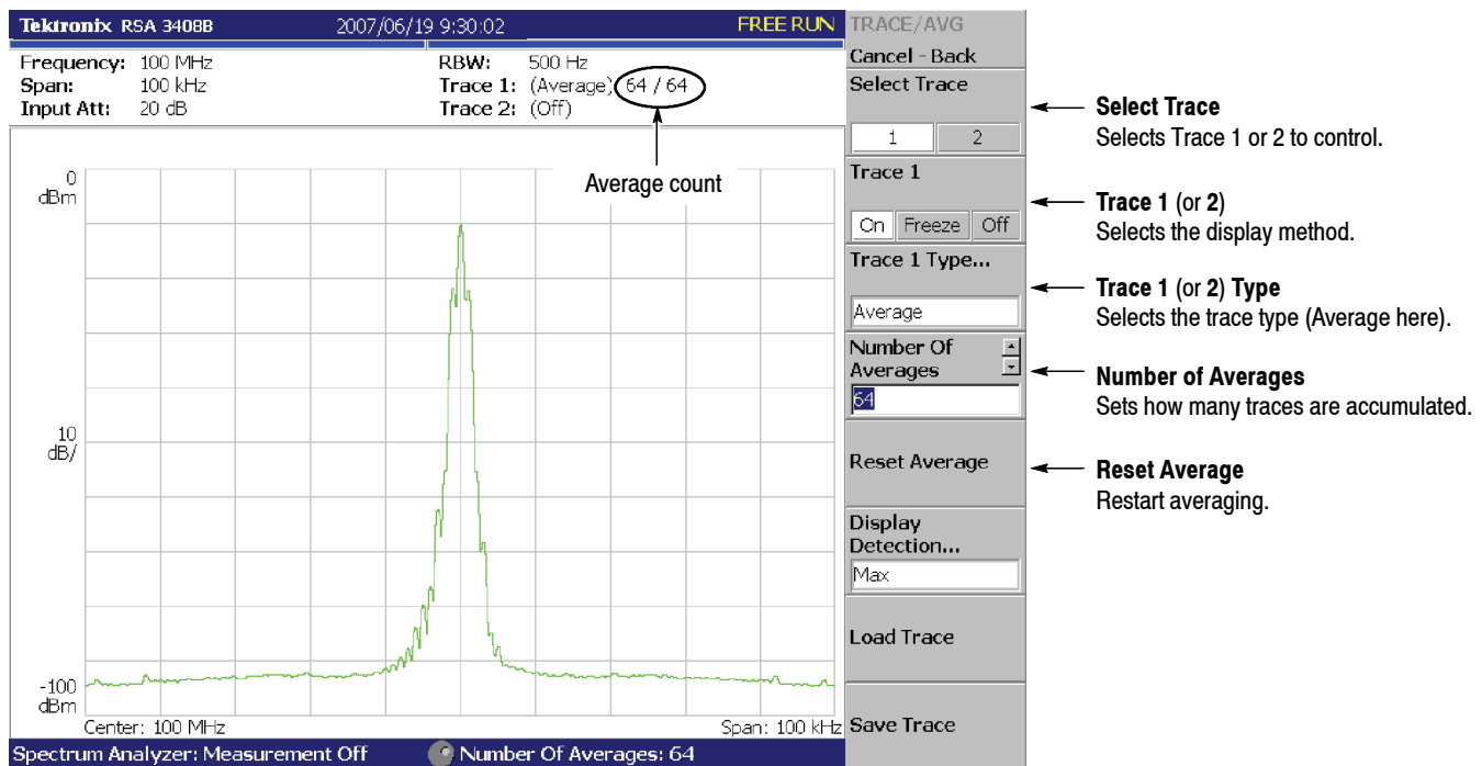
Figure 3-136: Displaying an averaged waveform
