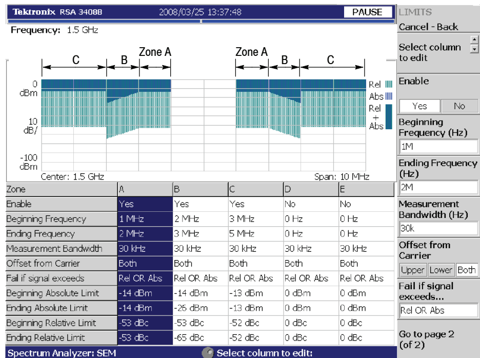
Figure 3-17: Measurement limits editor
