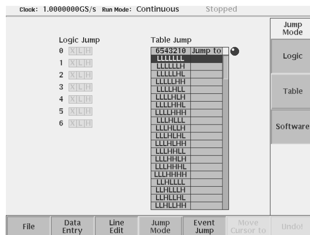
AWG710B
